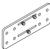
spreader plate A face fixture 430 × 160 × 12 mm
